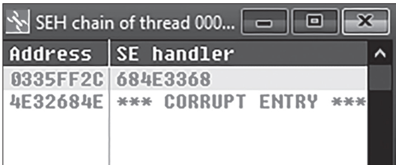
Figure 14-3: The SEH overwritten with random characters
