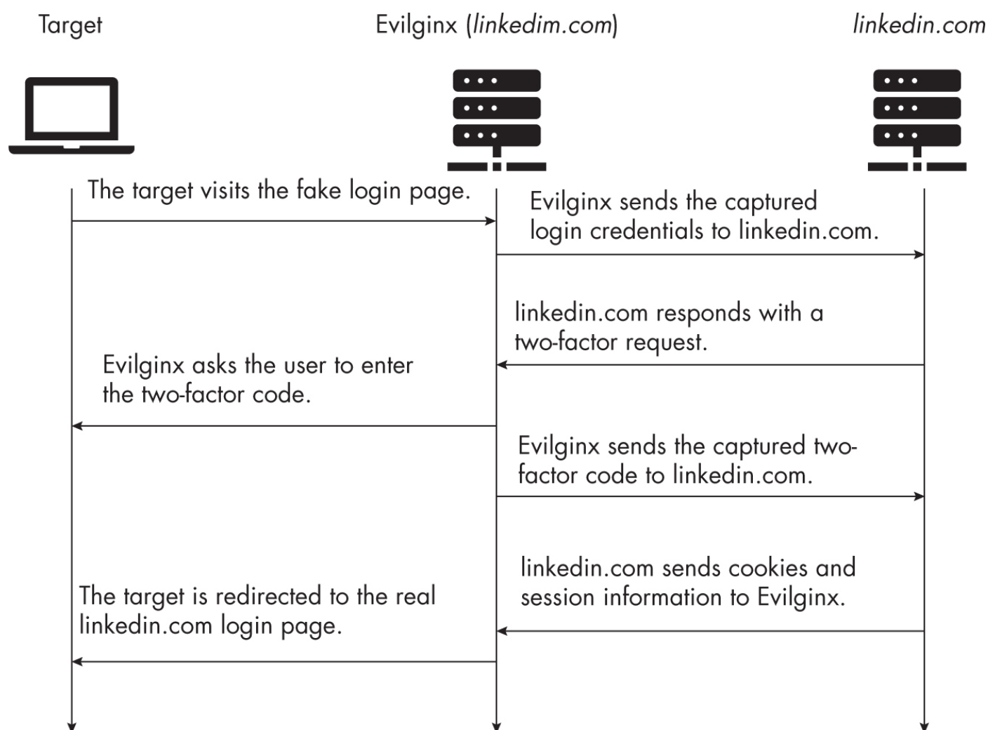
Figure 8-1: How Evilginx bypasses two-factor authentication
