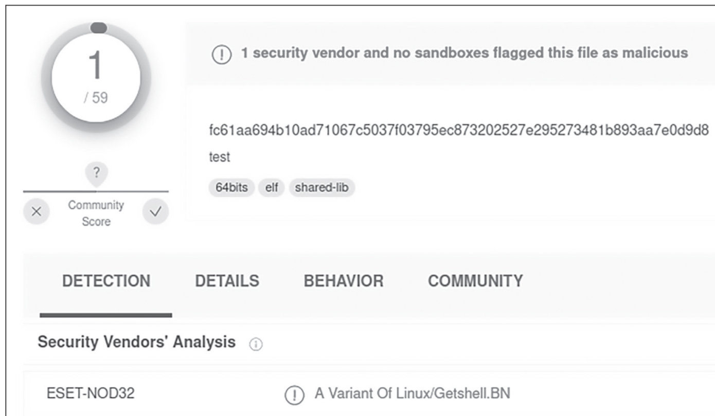
Figure 7-6: Uploading the compiled custom program to VirusTotal
