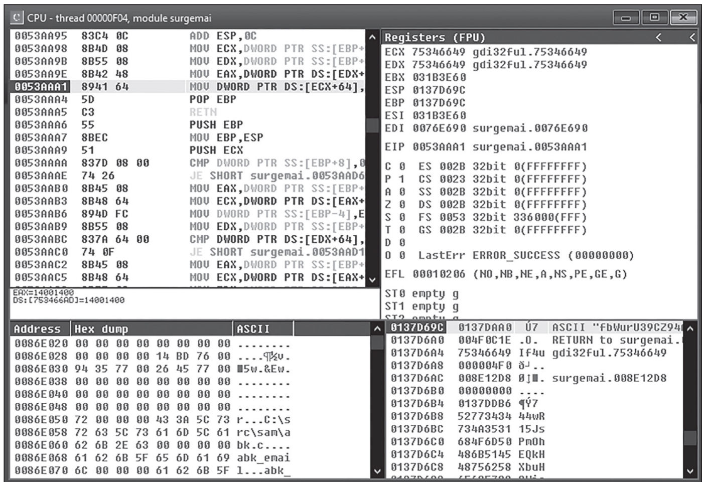
Figure 14-1: The debugger paused at the point of the crash
