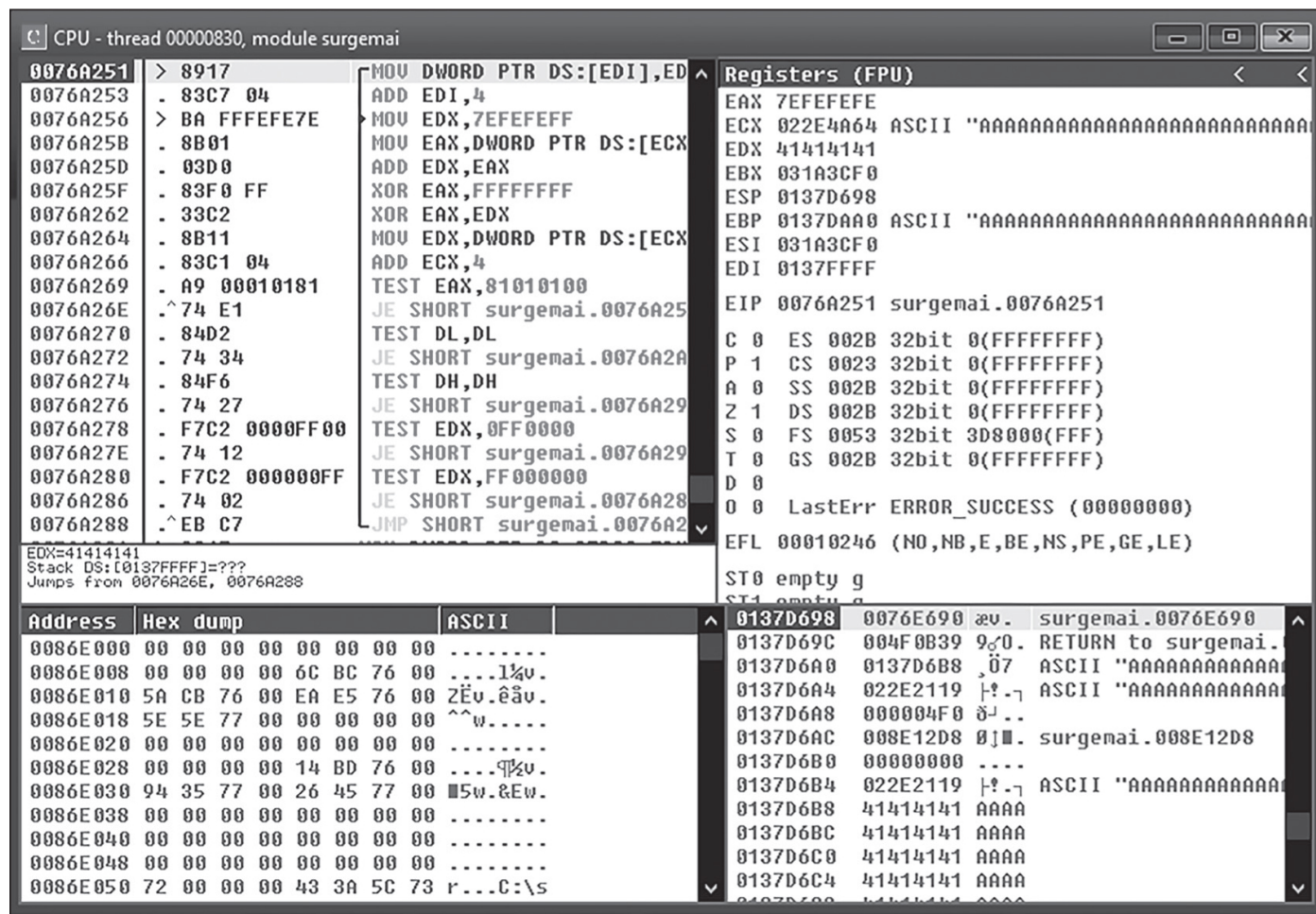
Figure 14-2: The overwritten SEH entry
