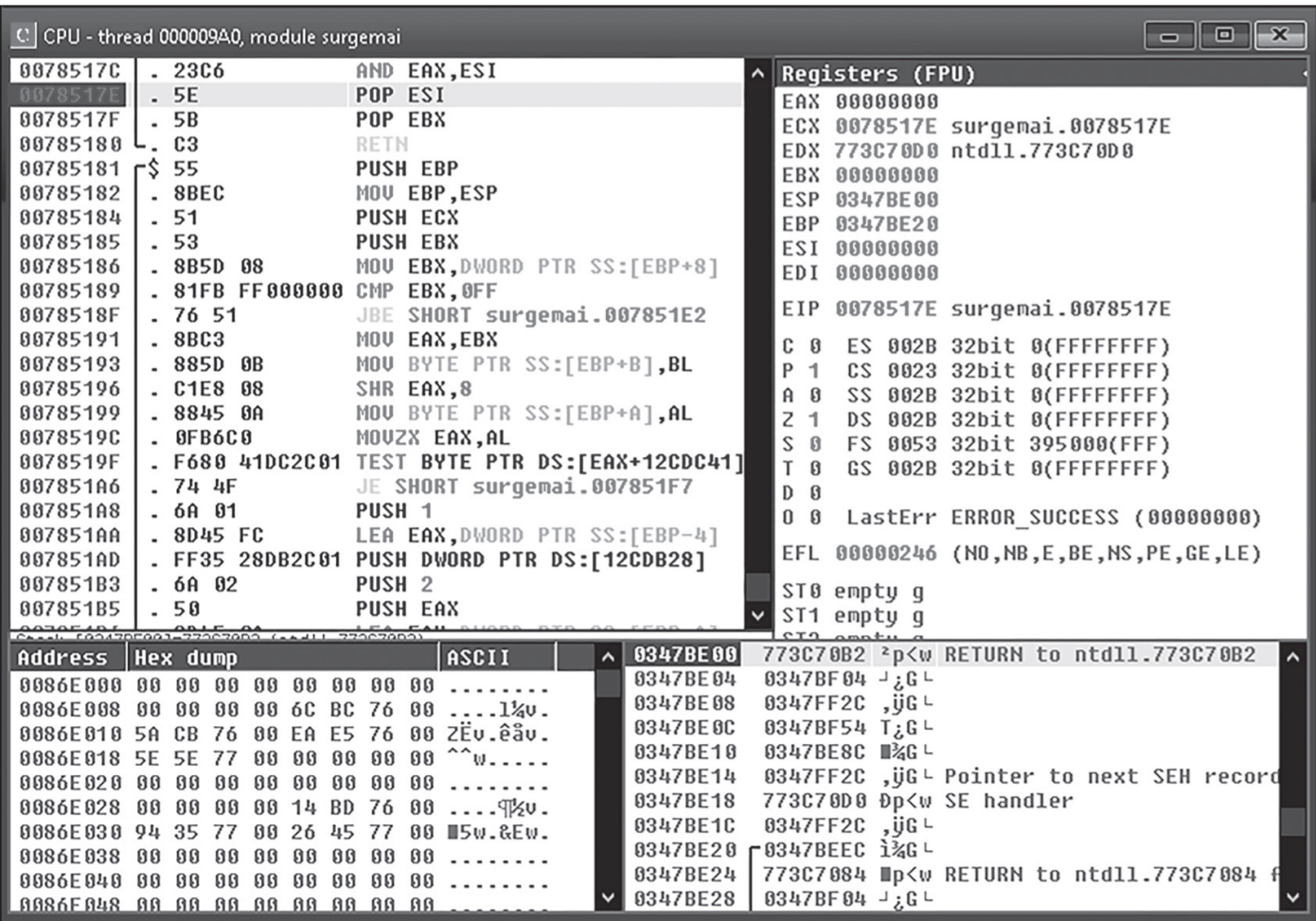
Figure 14-4: Landing in the POP-POP-RETN instructions
